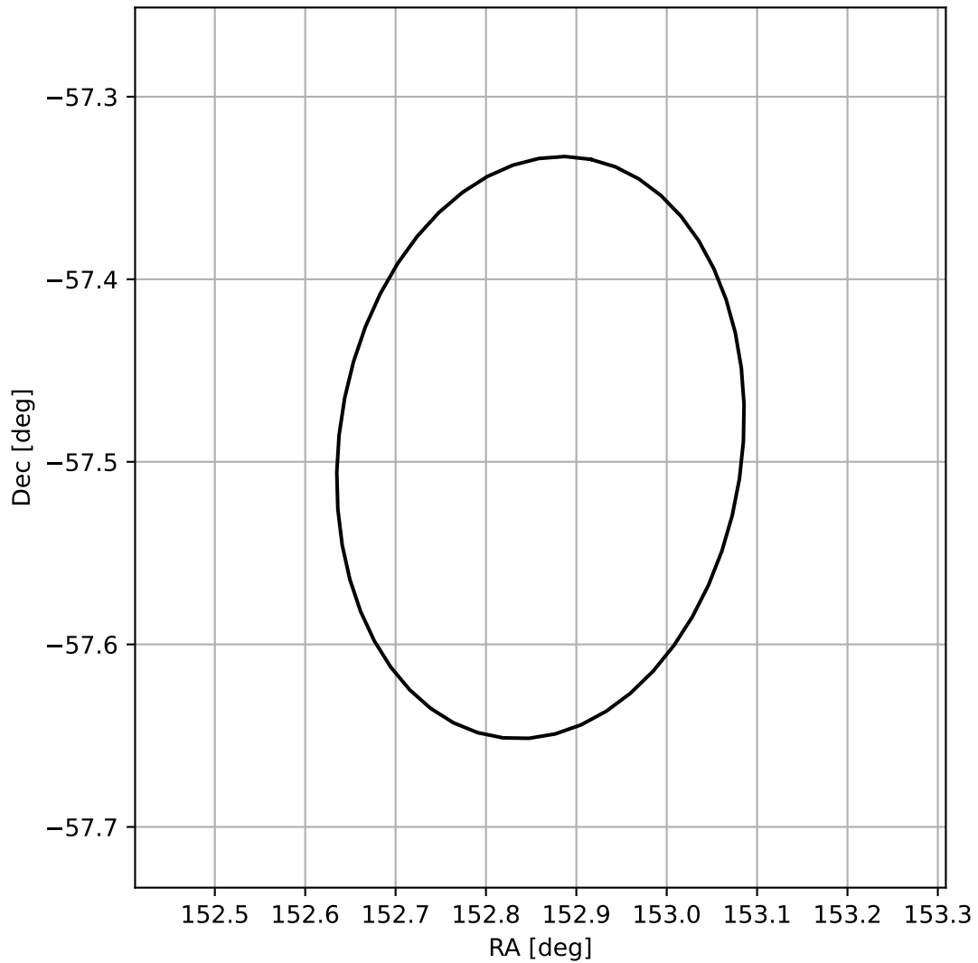
4FGL J1011.4-5729
