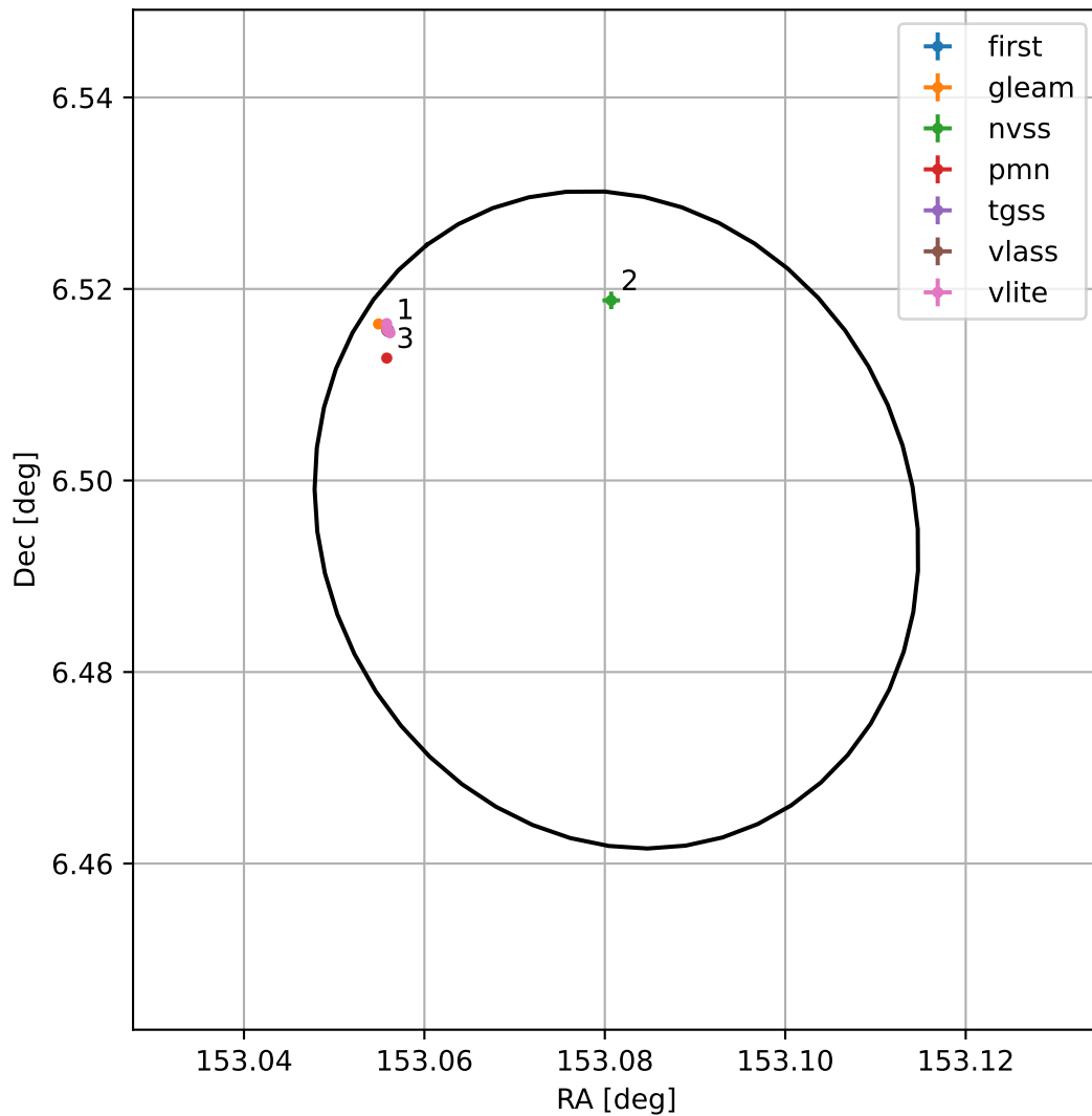
4FGL J1012.3+0629
