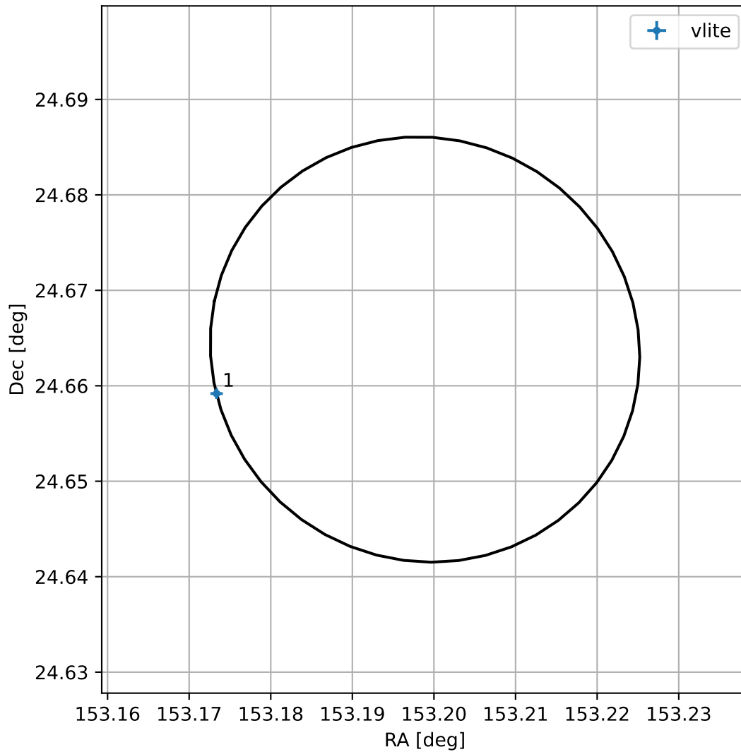
4FGL J1012.7+2439
