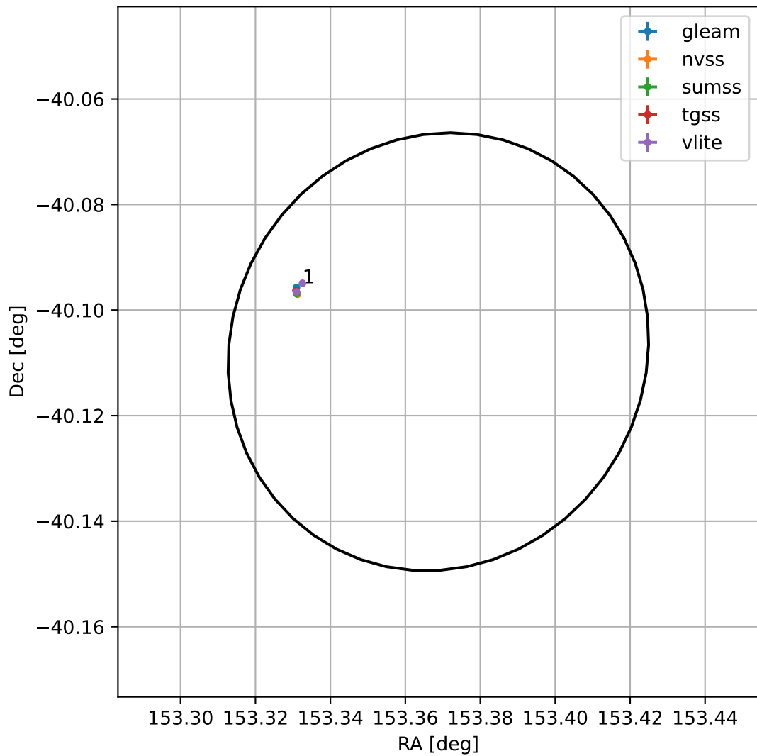
4FGL J1013.4-4006
