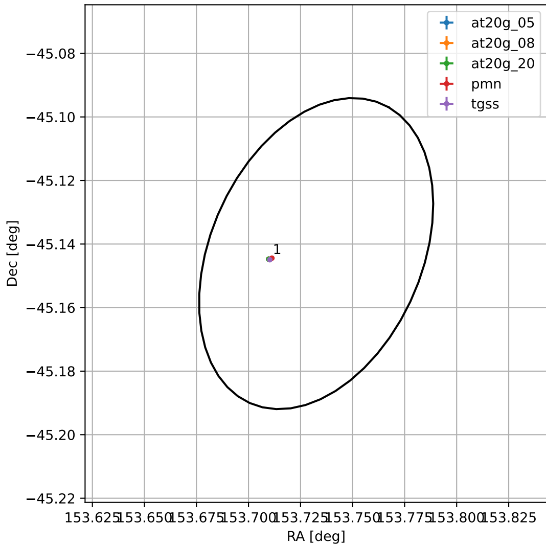
4FGL J1014.9-4508
