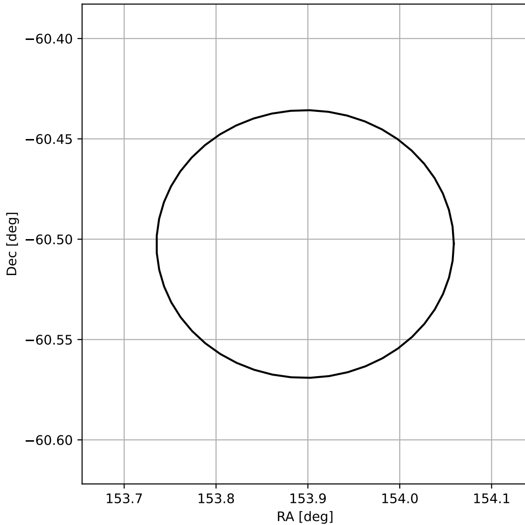
4FGL J1015.5-6030
