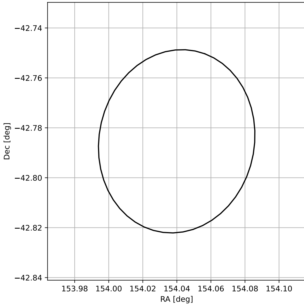
4FGL J1016.1-4247
