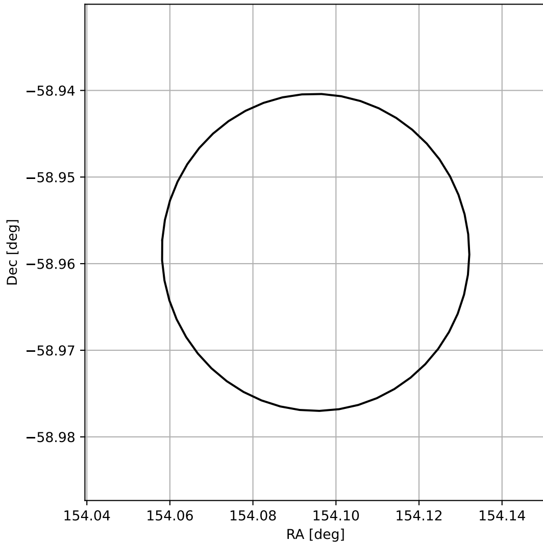
4FGL J1016.3-5857
