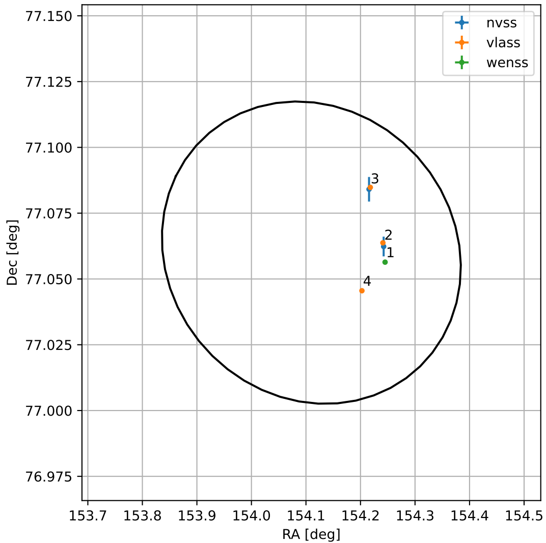
4FGL J1016.4+7703
