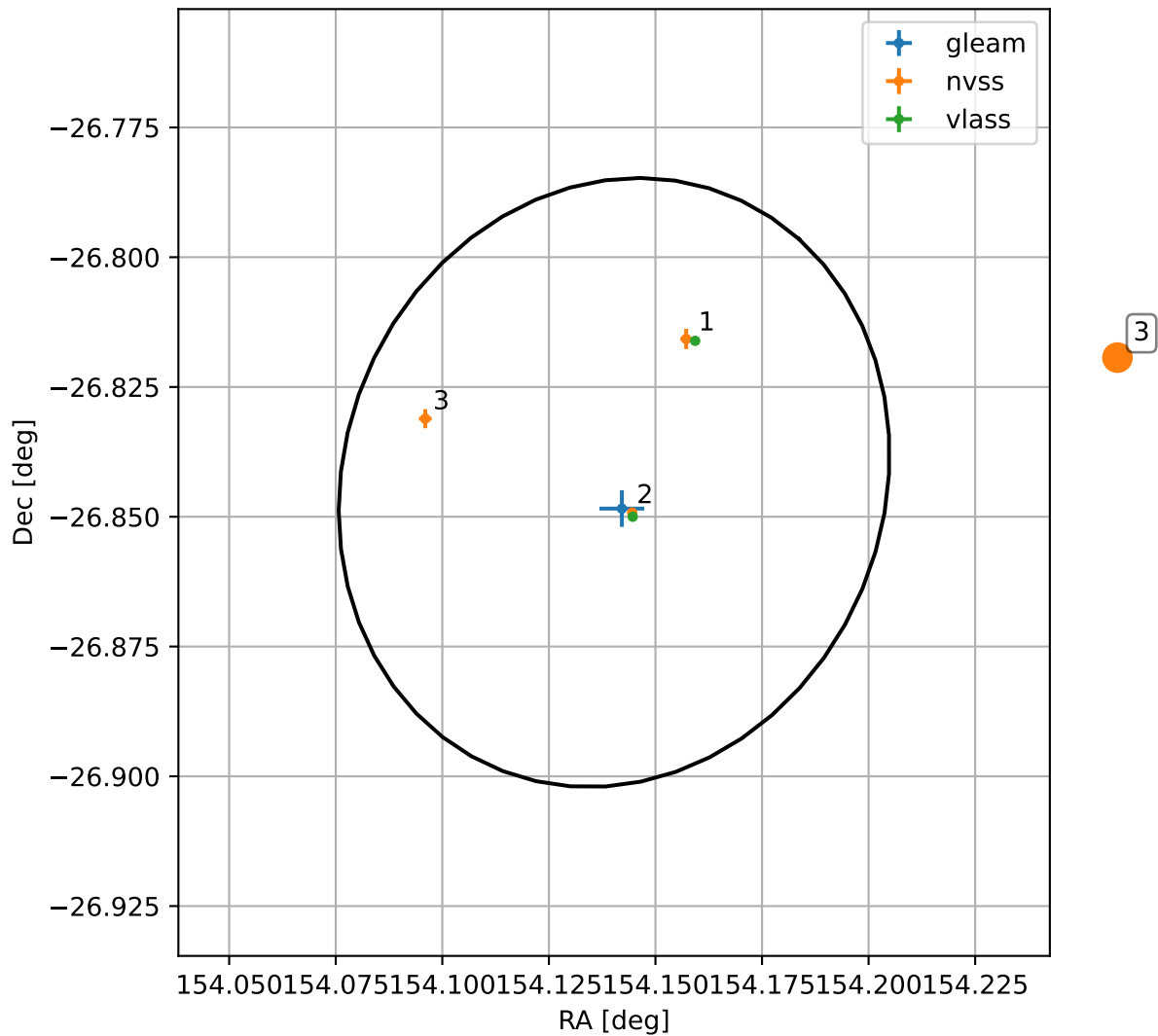
4FGL J1016.5-2650
