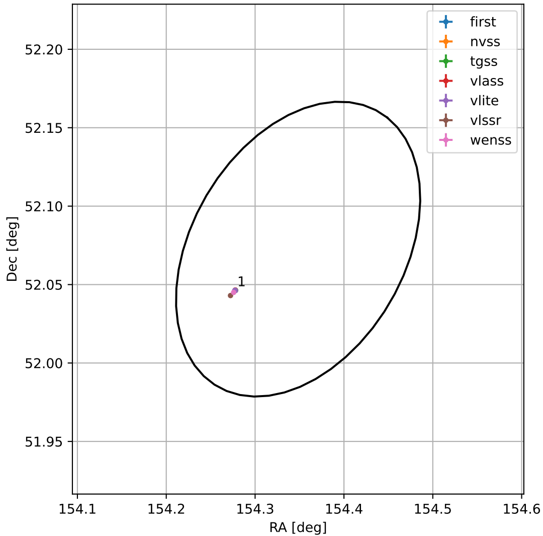
4FGL J1017.3+5204
