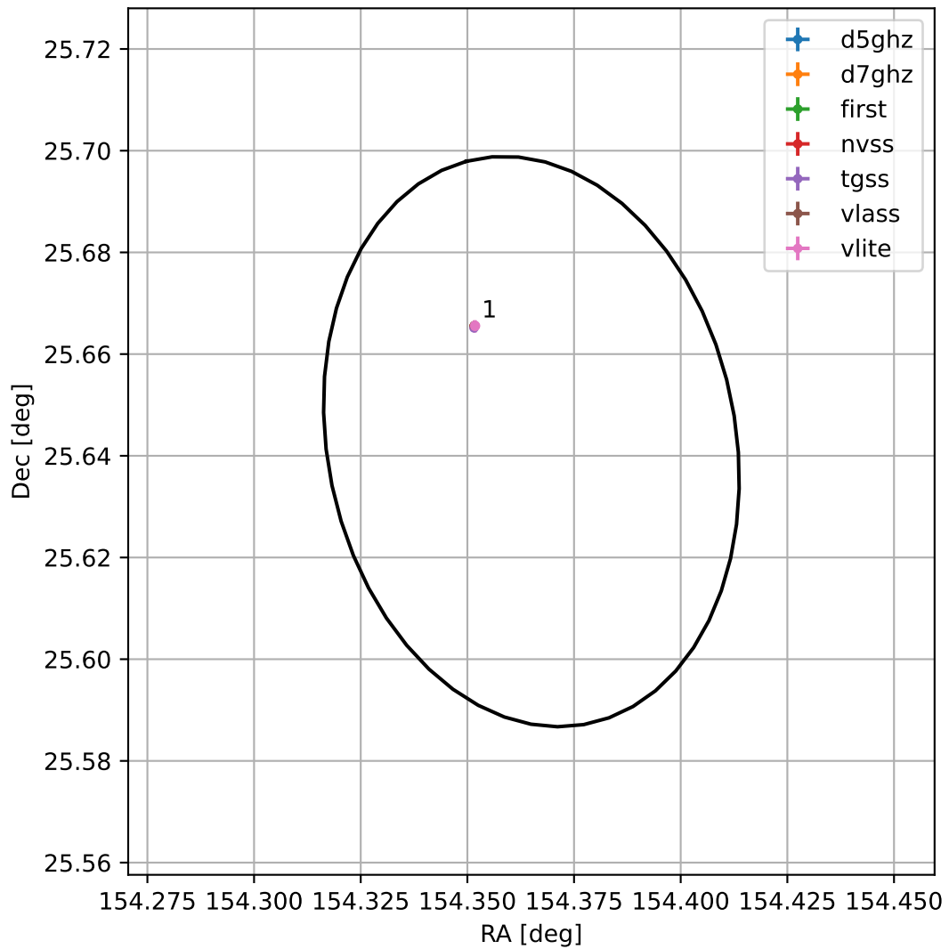
4FGL J1017.4+2538
