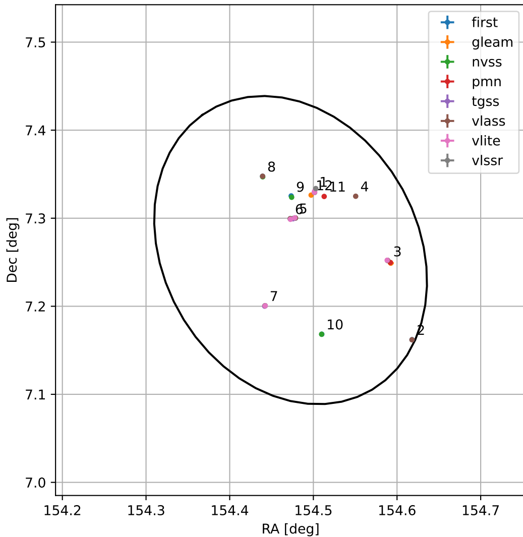
4FGL J1017.8+0715
