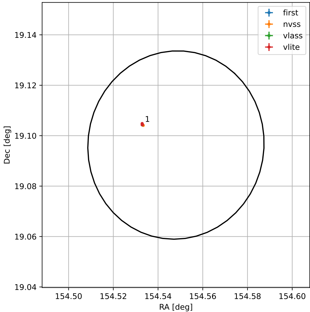
4FGL J1018.1+1905
