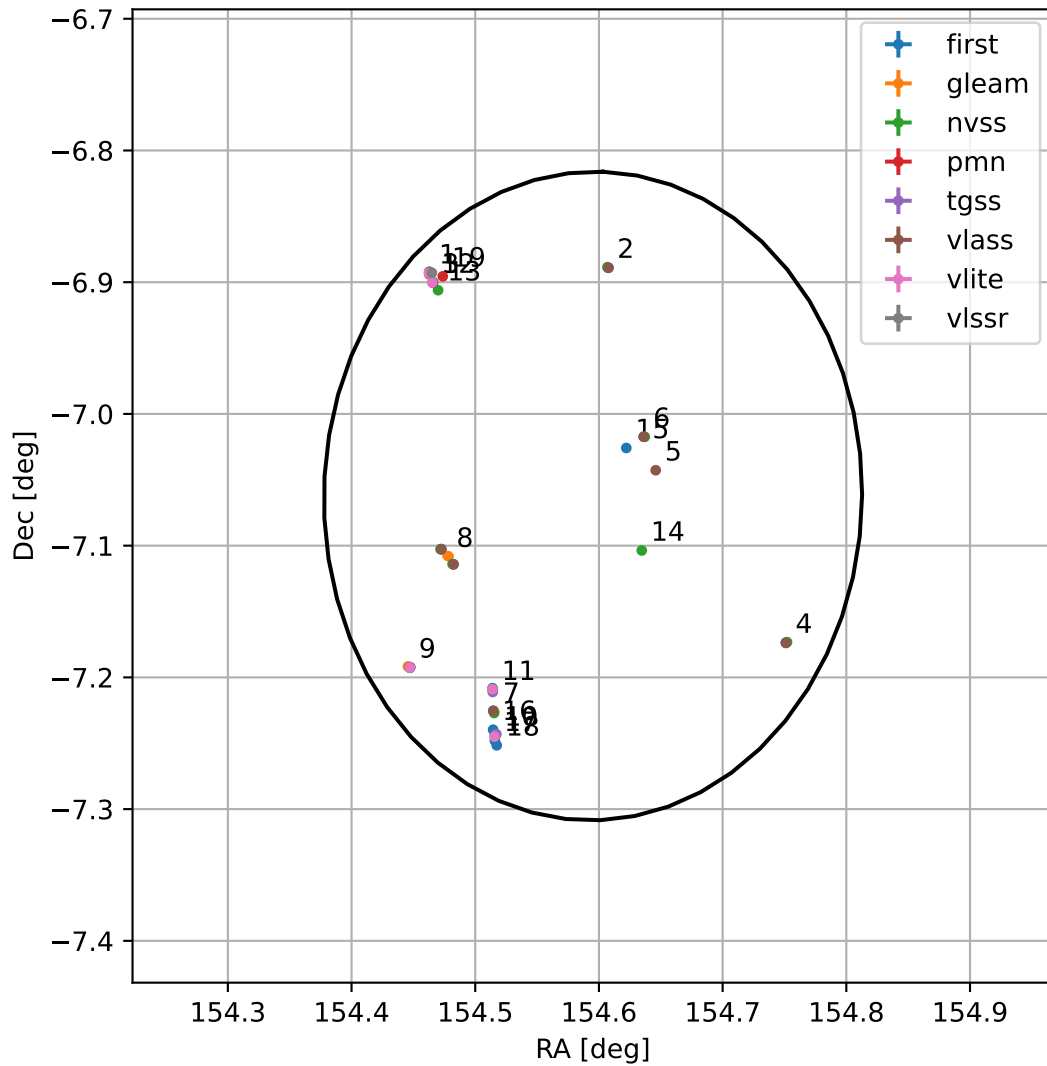
4FGL J1018.3-0703
