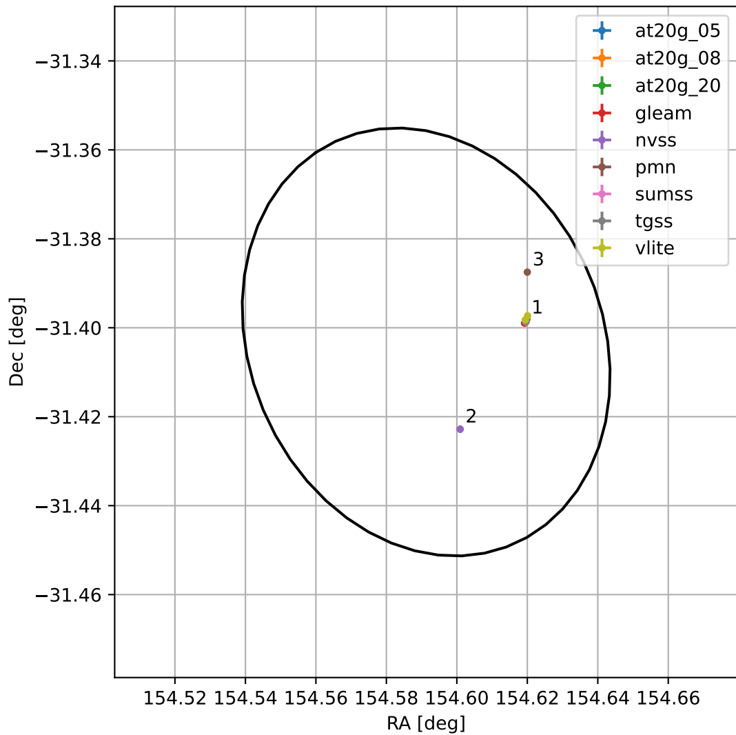
4FGL J1018.3-3124
