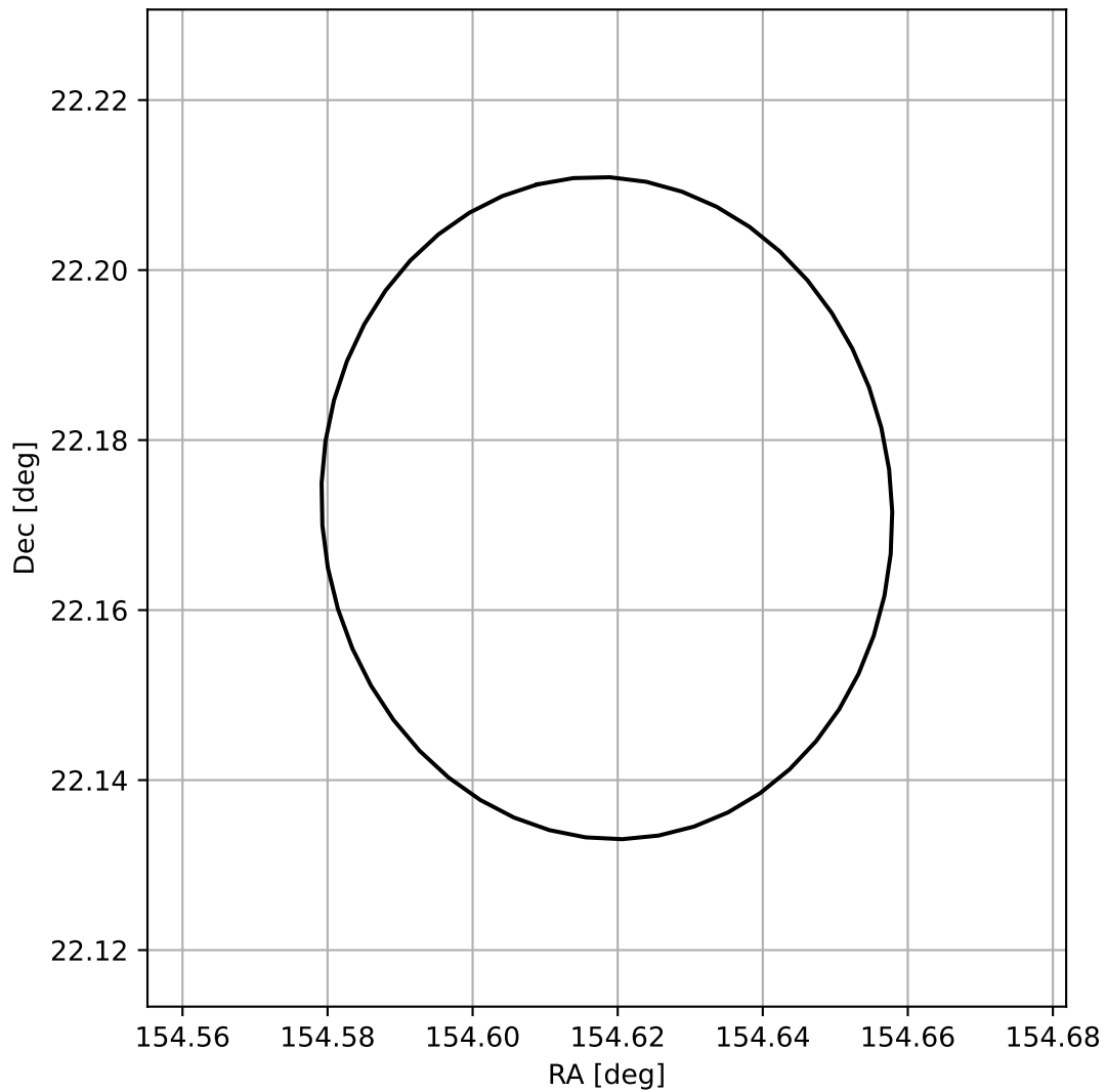
4FGL J1018.4+2210
