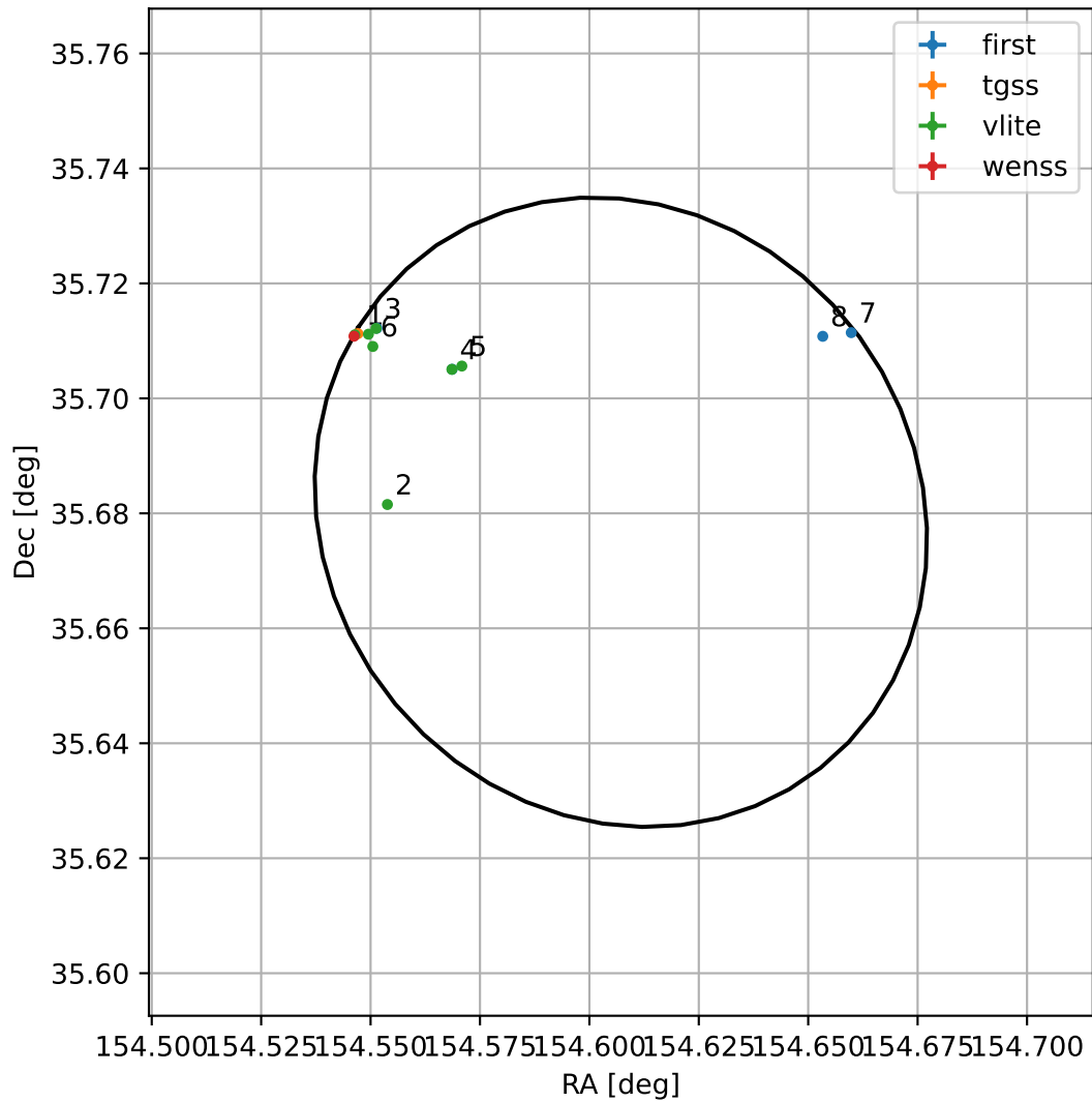
4FGL J1018.4+3540
