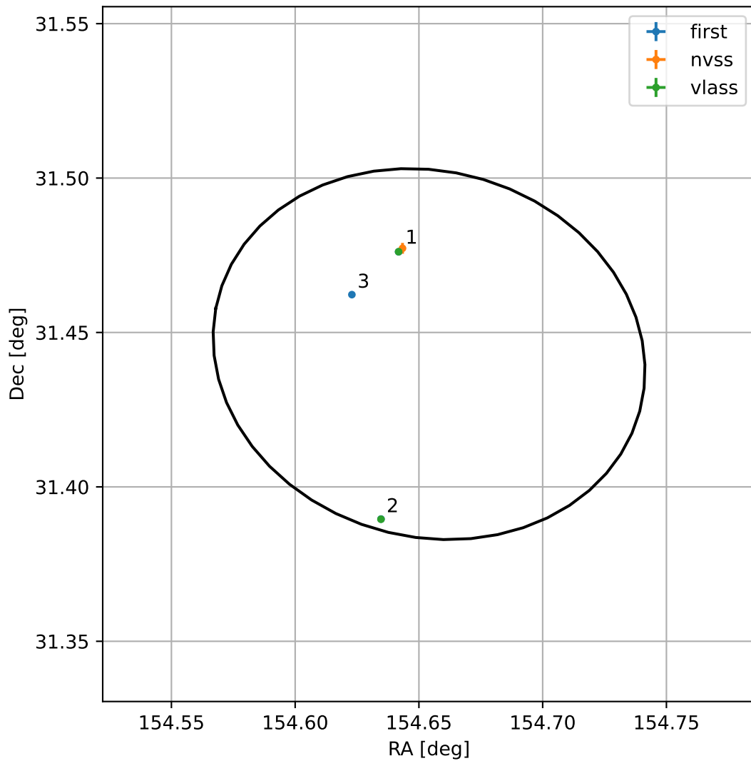
4FGL J1018.6+3126
