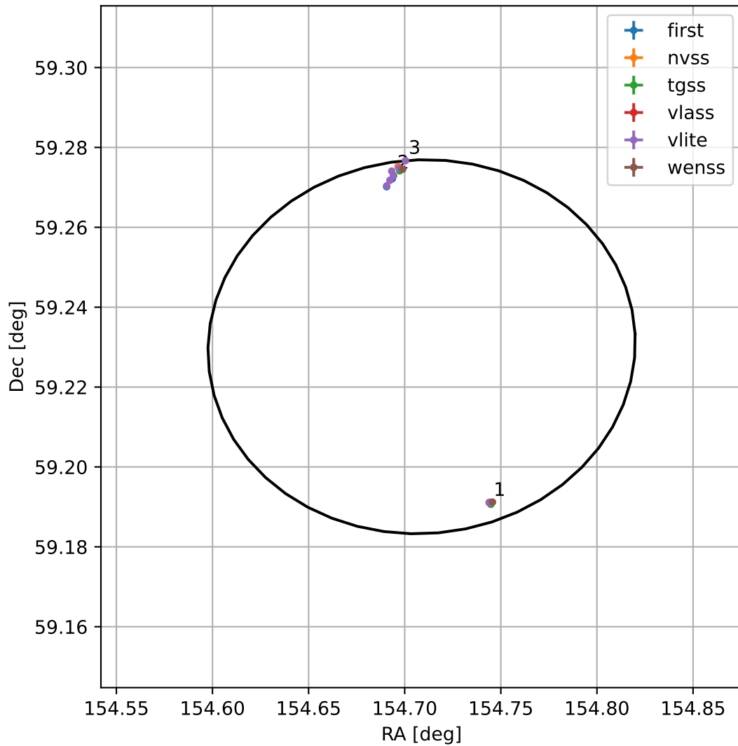
4FGL J1018.8+5913
