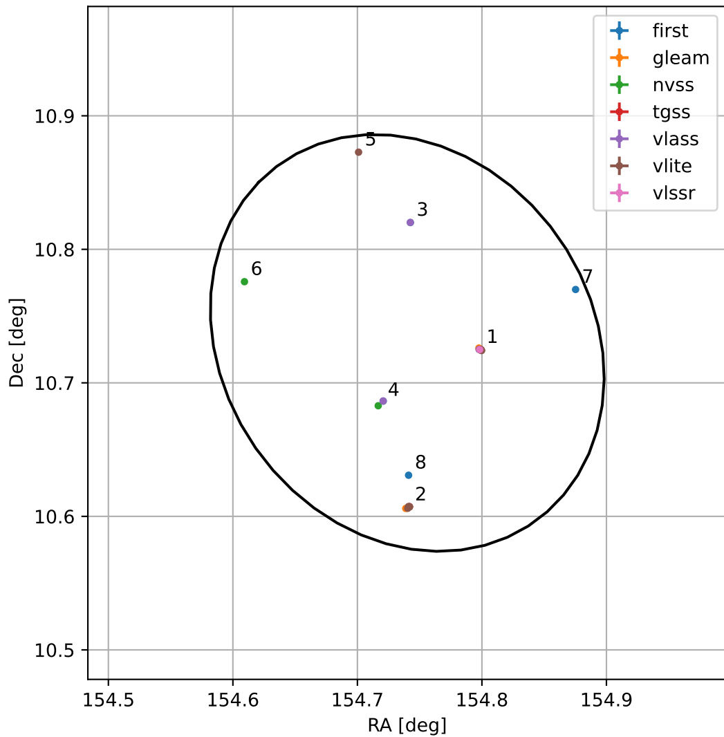
4FGL J1018.9+1043
