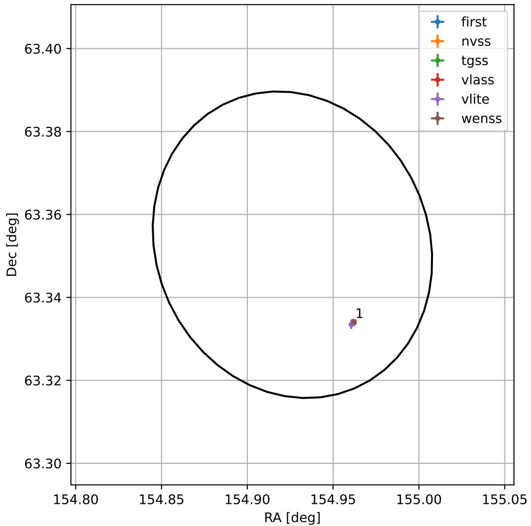
4FGL J1019.7+6321
