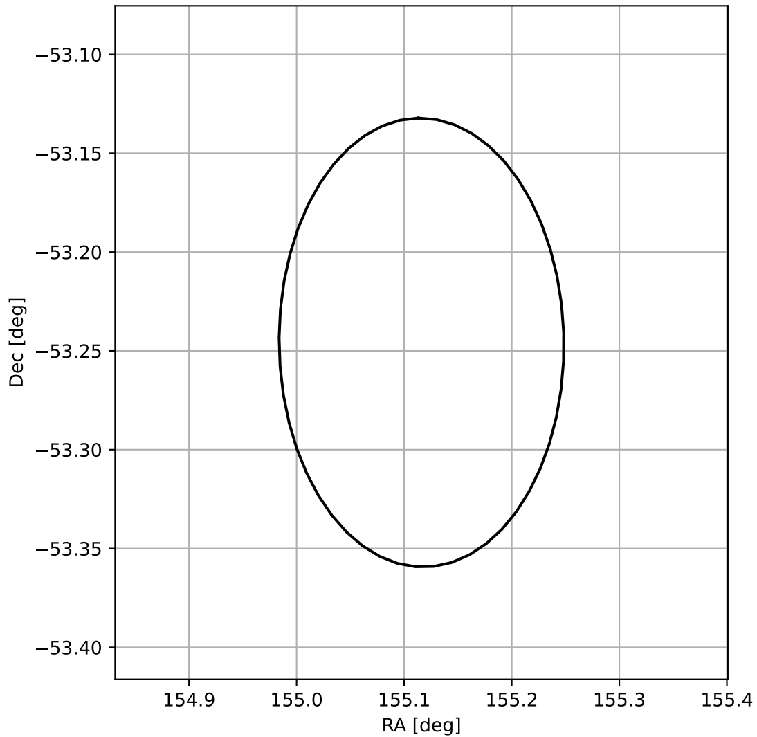
4FGL J1020.4-5314
