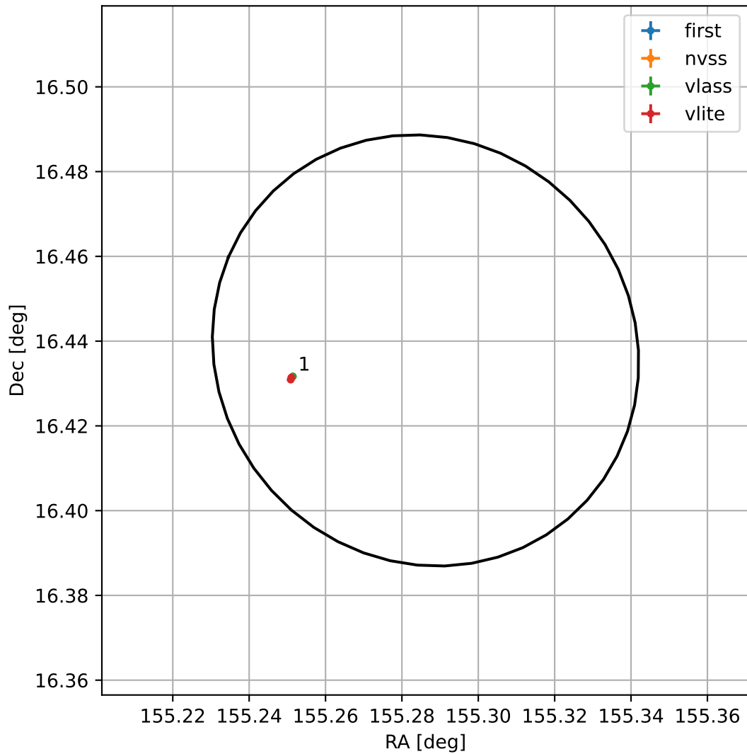
4FGL J1021.1+1626
