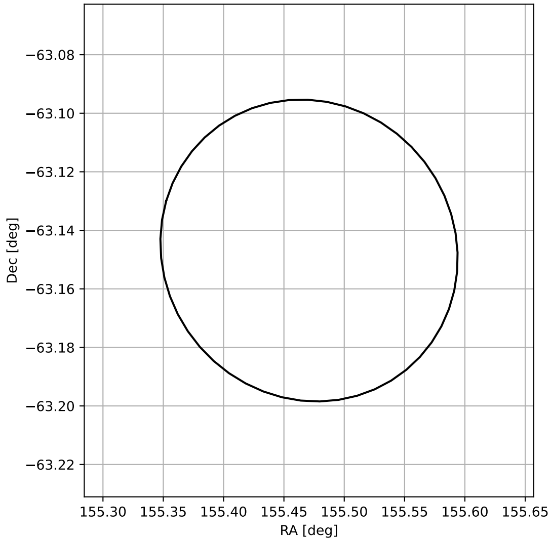
4FGL J1021.8-6308
