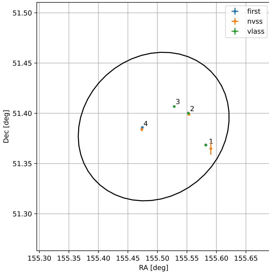
4FGL J1021.9+5123
