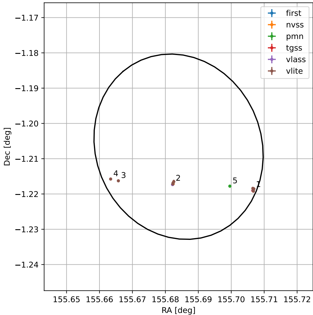
4FGL J1022.7-0112
