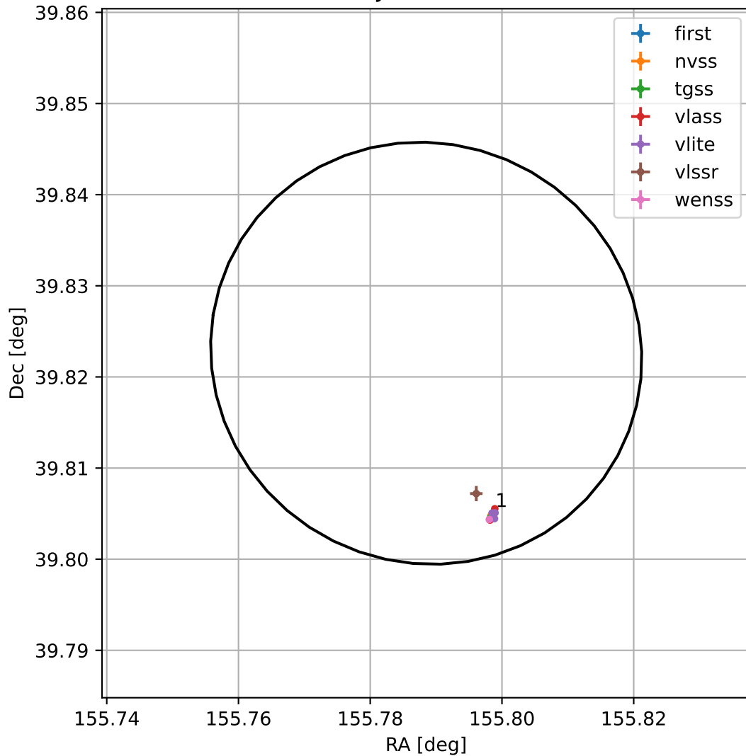
4FGL J1023.1+3949
