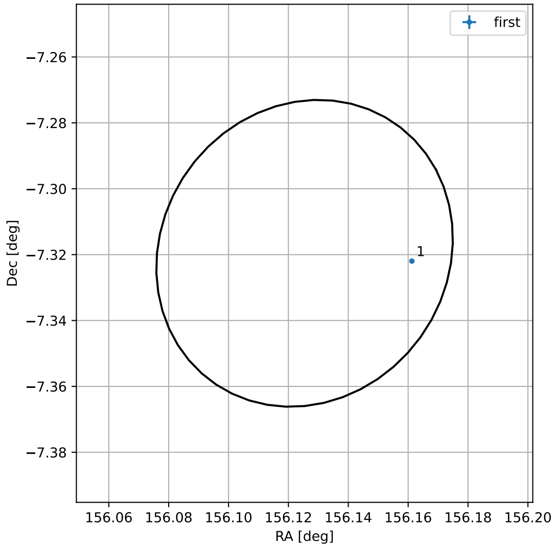
4FGL J1024.5-0719
