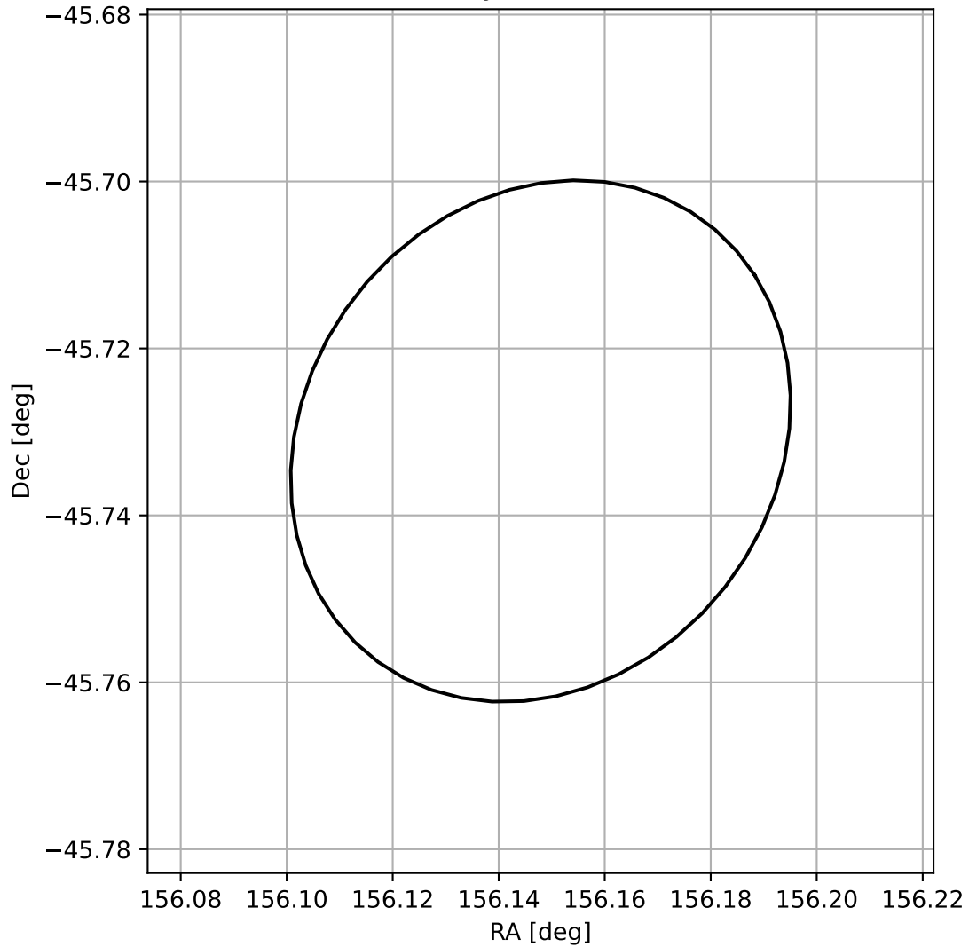
4FGL J1024.5-4543
