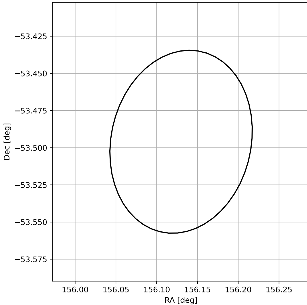
4FGL J1024.5-5329
