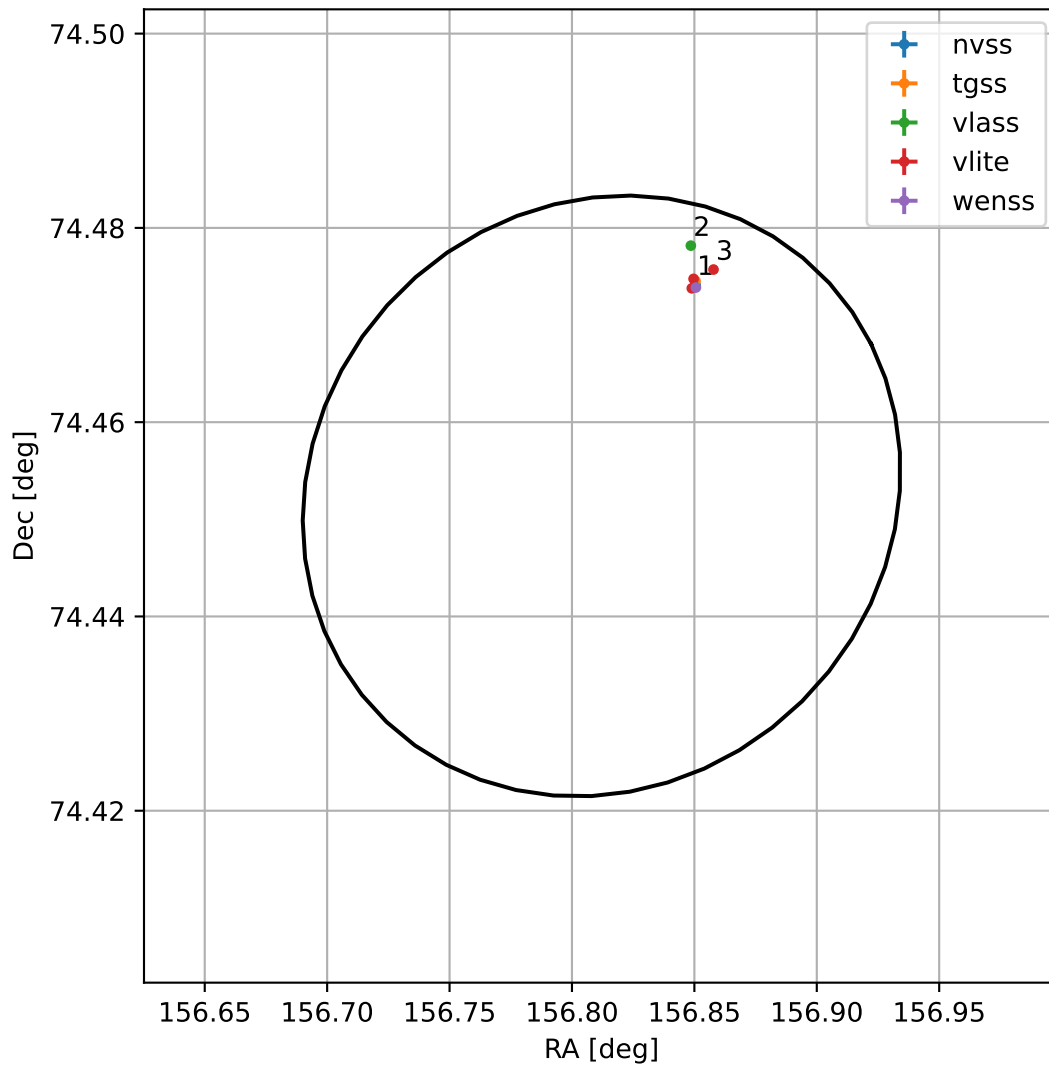
4FGL J1027.2+7427
