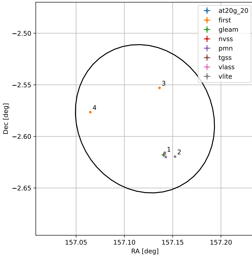
4FGL J1028.4-0234
