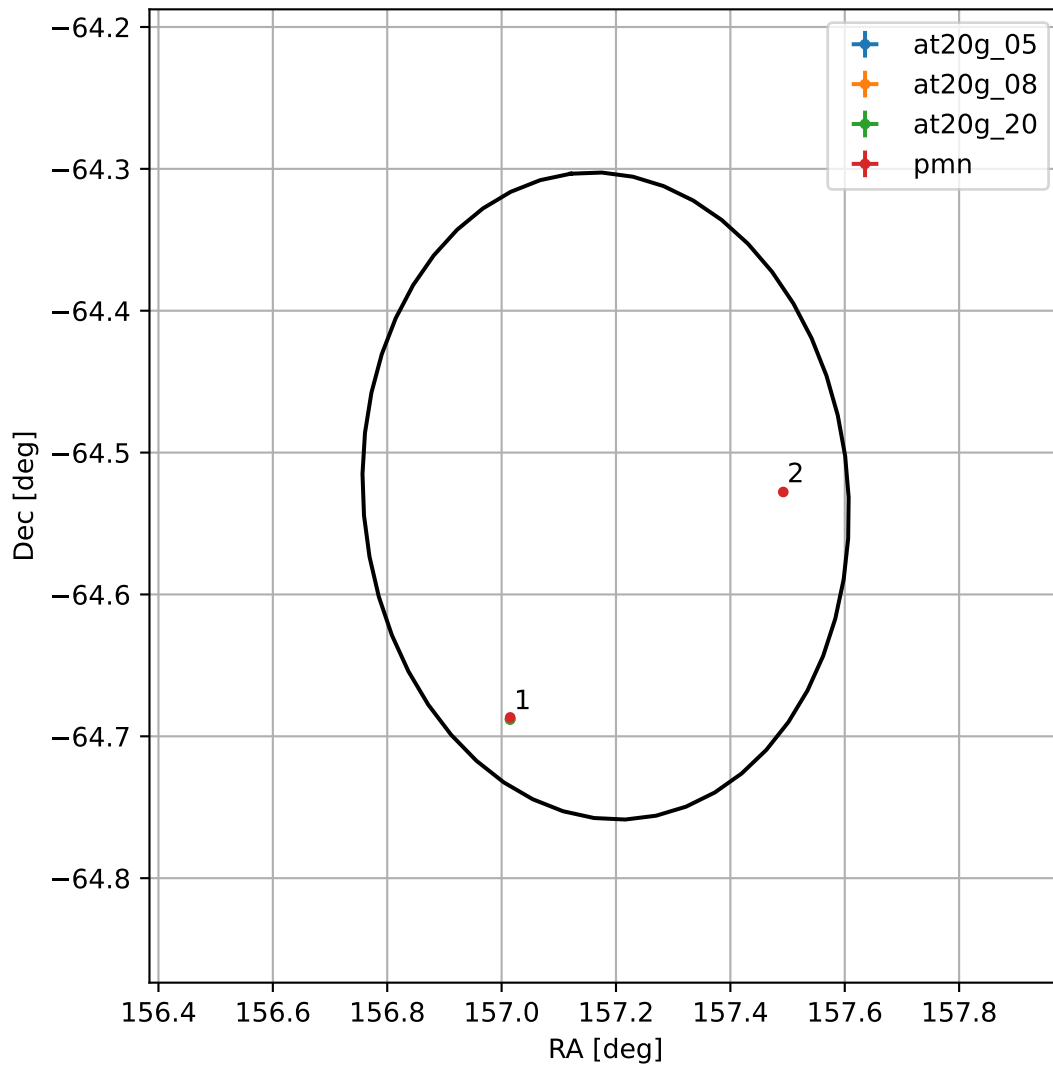
4FGL J1028.7-6431
