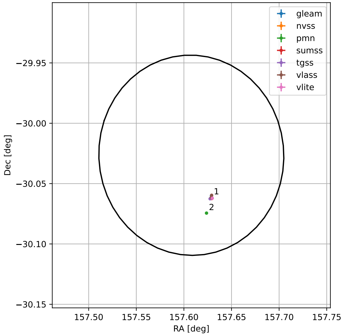
4FGL J1030.4-3001
