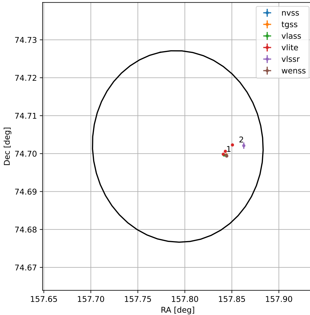
4FGL J1031.1+7442
