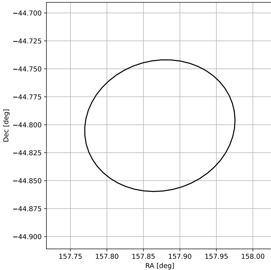
4FGL J1031.4-4448
