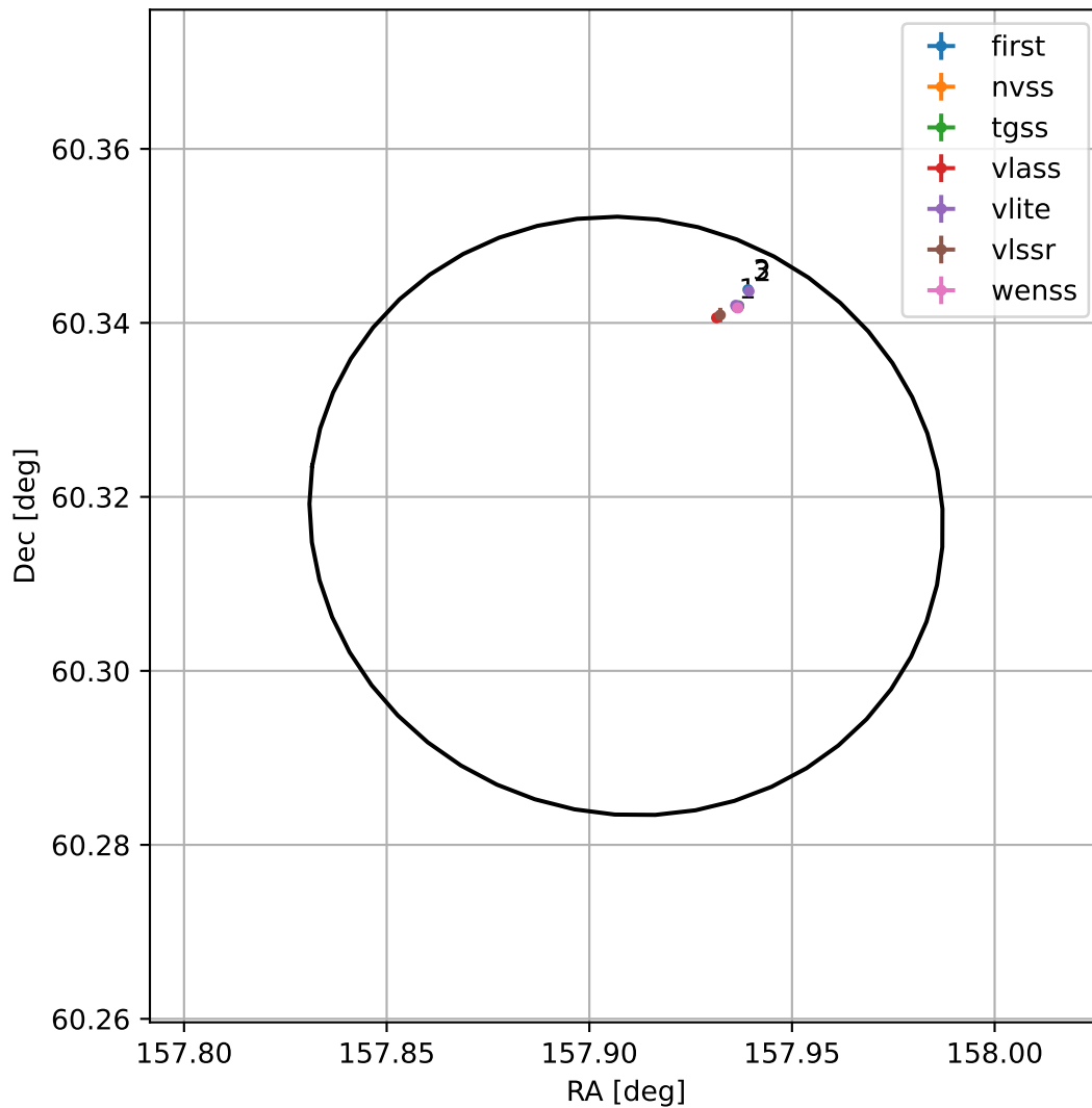
4FGL J1031.6+6019
