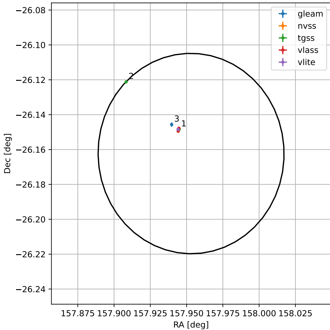
4FGL J1031.8-2609
