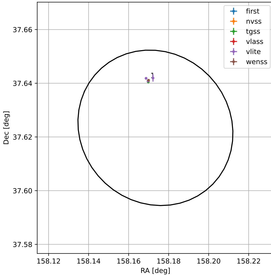
4FGL J1032.6+3737
