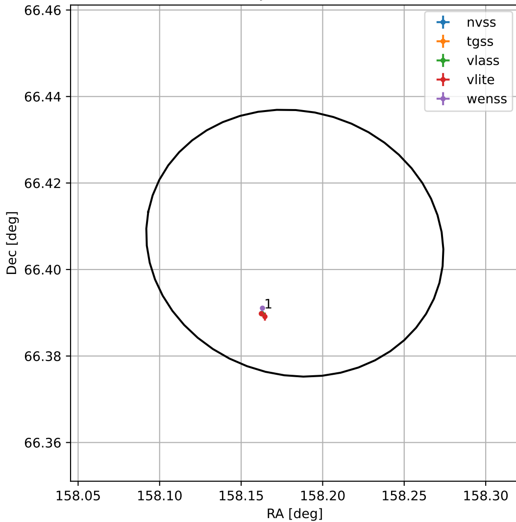
4FGL J1032.7+6624
