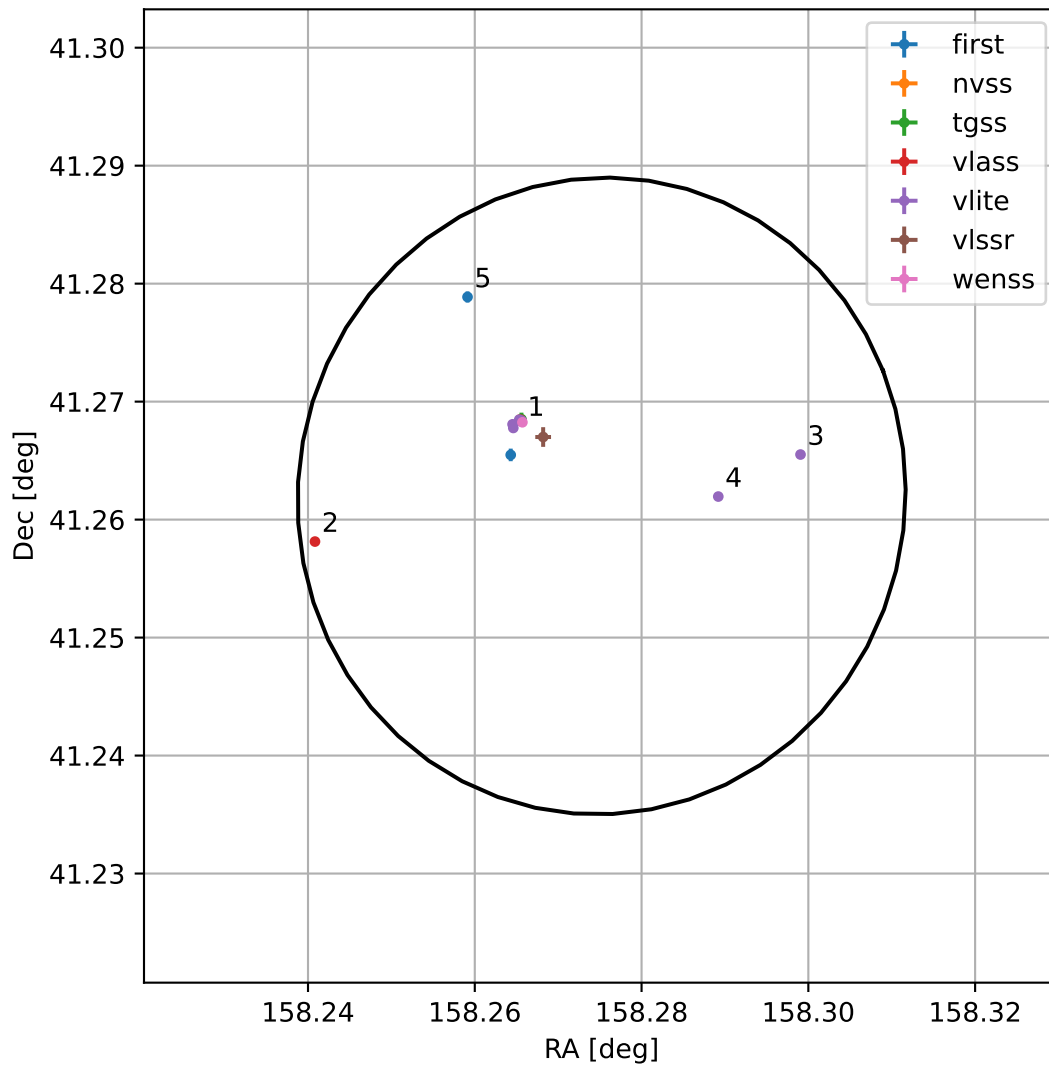
4FGL J1033.1+4115
