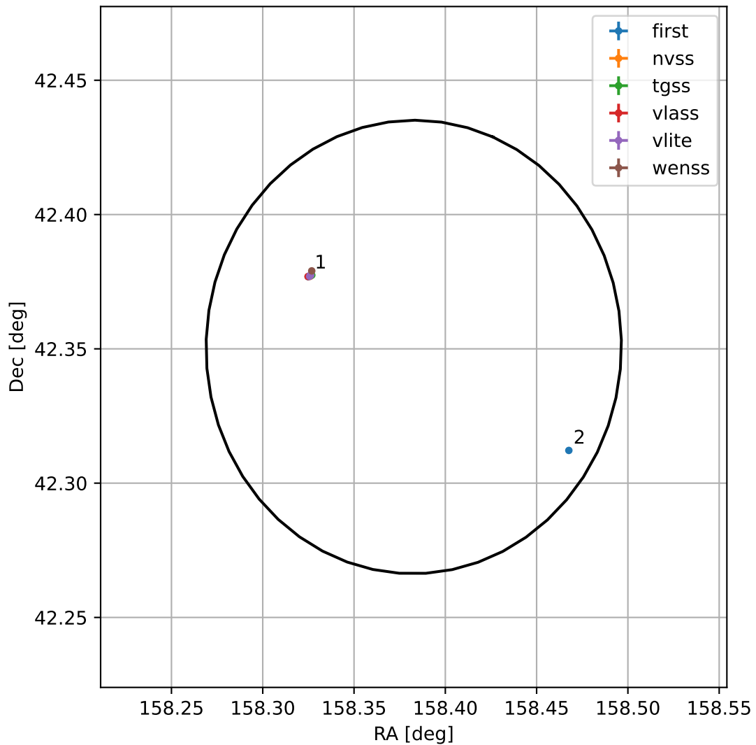
4FGL J1033.5+4221
