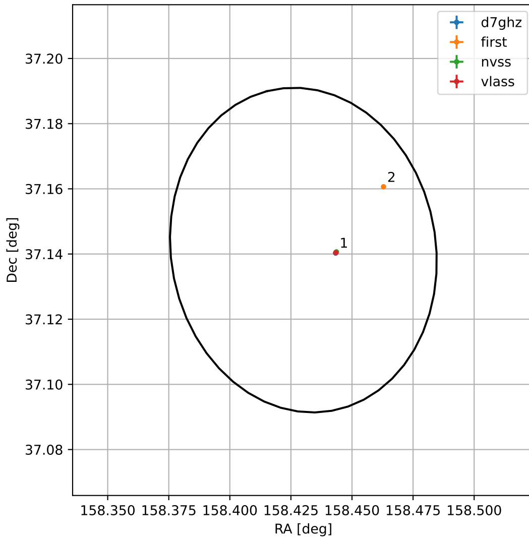
4FGL J1033.7+3708
