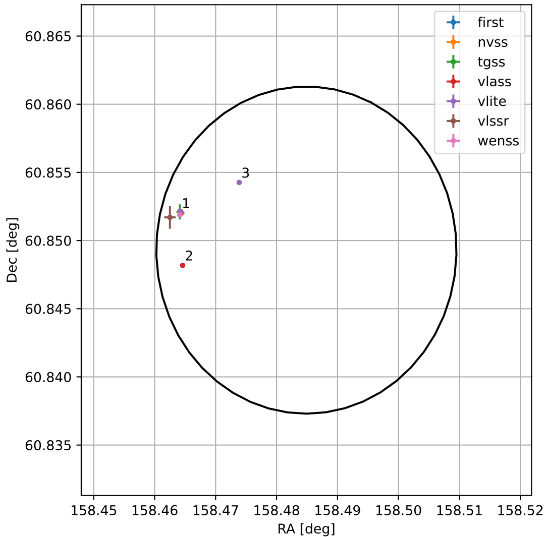
4FGL J1033.9+6050
