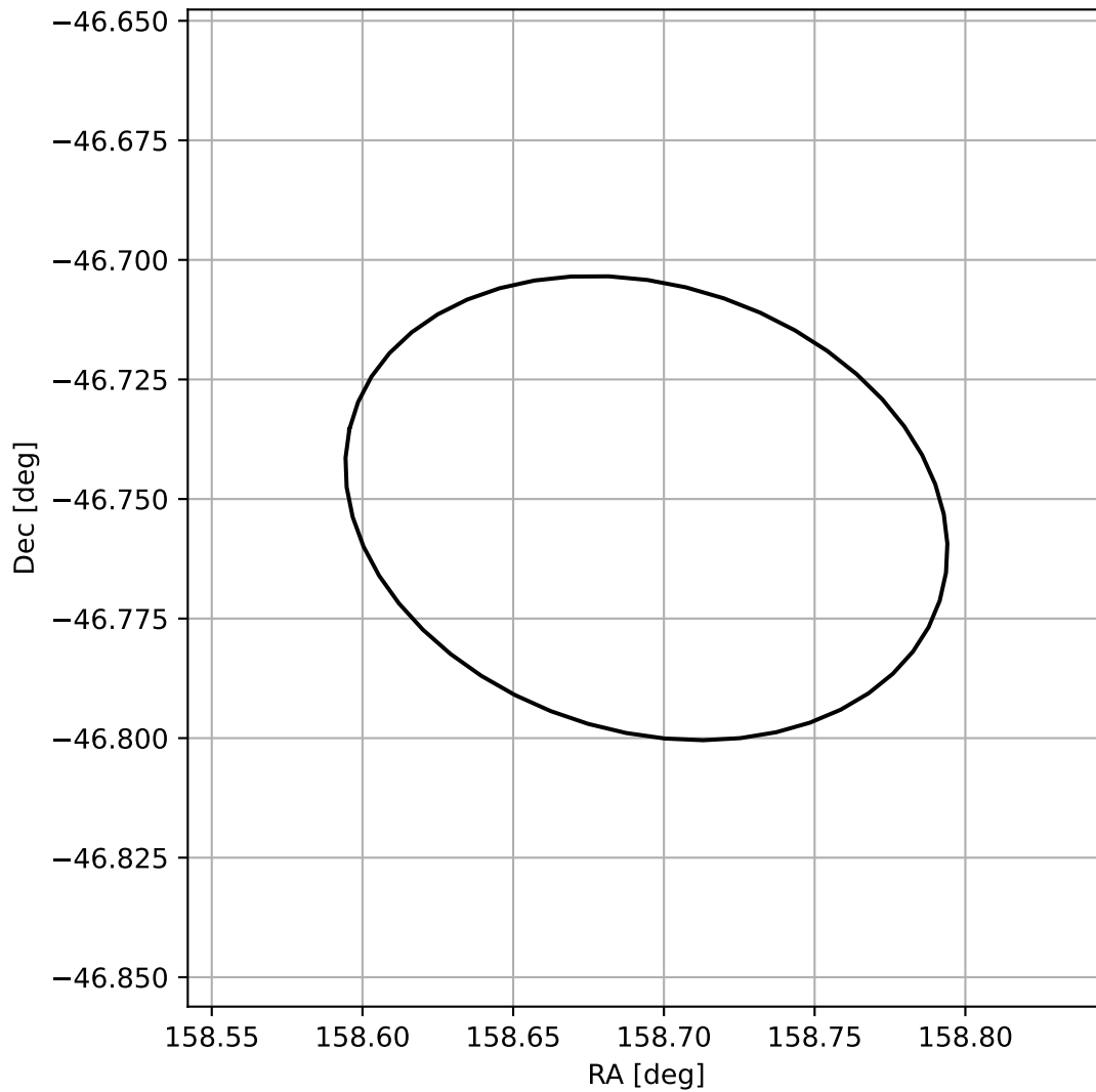
4FGL J1034.7-4645
