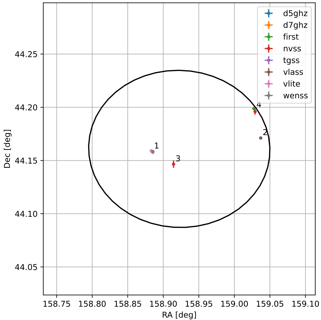
4FGL J1035.6+4409
