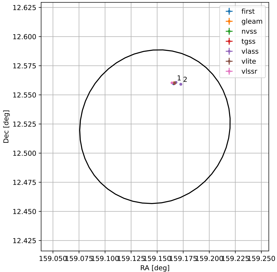
4FGL J1036.5+1231
