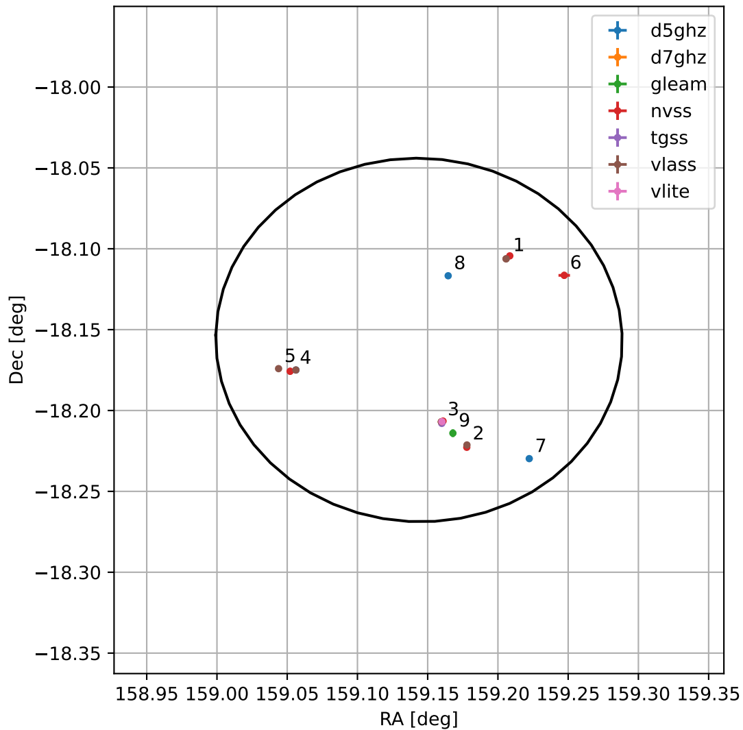
4FGL J1036.5-1809
