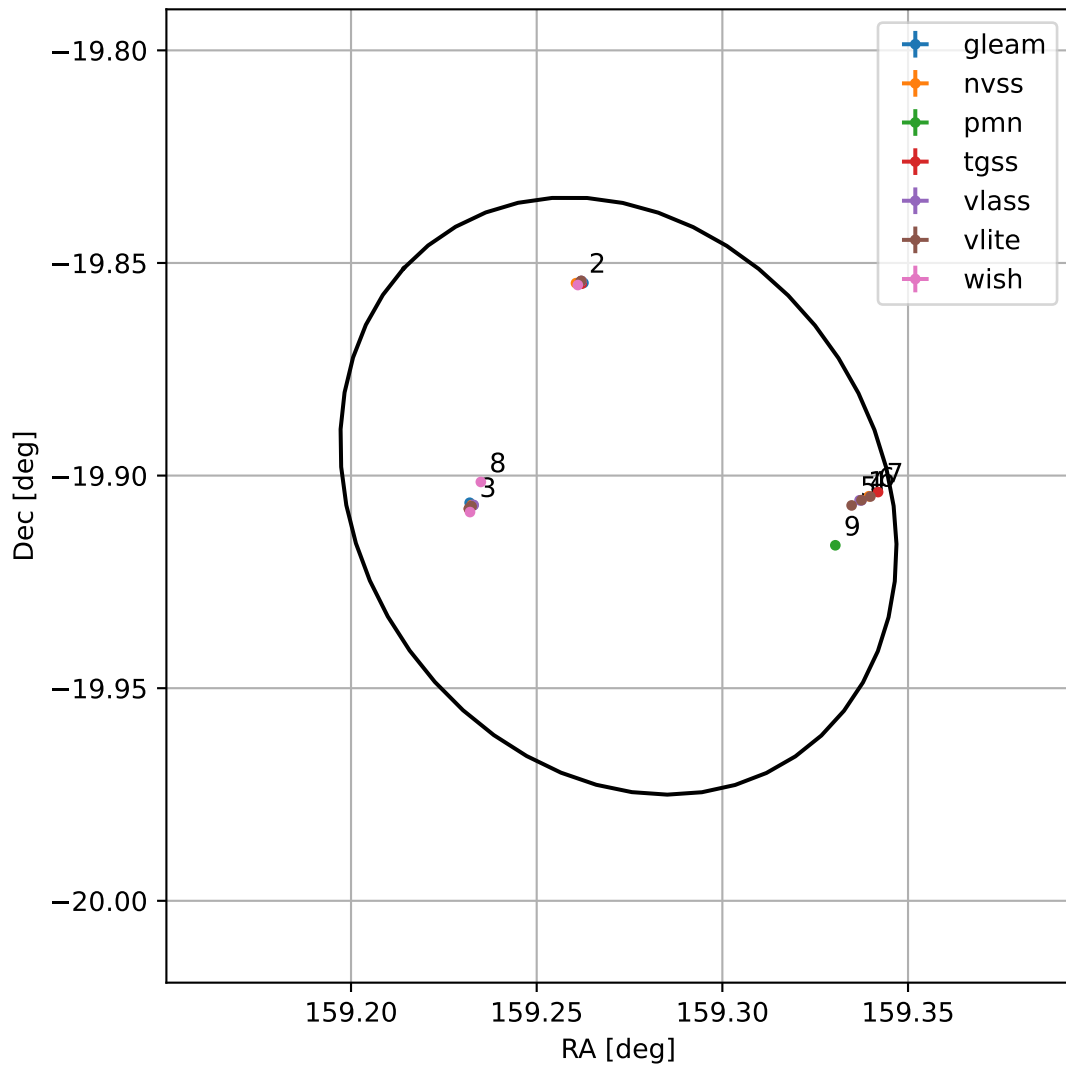
4FGL J1037.0-1954
